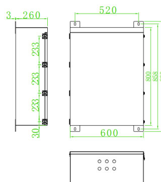
CM-HT12/G Structure chart
